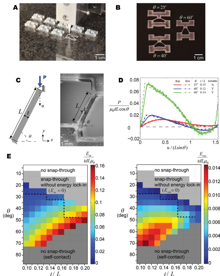
Figure 2. Mechanical response of a constrained, tilted elastic beam. a) Minimal functional structures, each with a unique combination of geometrical parameters, are rapidly printed (150–200 s each) using direct write 3D printing. b) Minimal structures consisting of two identical tilted beams. c) Schematic view showing the 2D model used in our FE simulations (left) and the corresponding beam in the fabricated minimal unit (right). d) Numerical and experimental force–displacement curves for three beams characterized by (\theta, t/L) = (25^\circ, 0.15) , (40^\circ, 0.12) , (60^\circ, 0.14) . The force is normalized by \mu_0 L d \cos \theta ( d denoting the out-of-plane thickness of the samples), while the displacement is normalized by L \sin \theta . e) Effect of \theta and t/L on the energy absorbed by the elastic beam ( E_{in} ) and the energy cost for the beam to snap back to its undeformed configuration ( E_{out} ). The black dashed lines indicate the experimentally observed transition between the geometries that result in bistability and those that merely possess the snap-through instability, but are not bistable.
